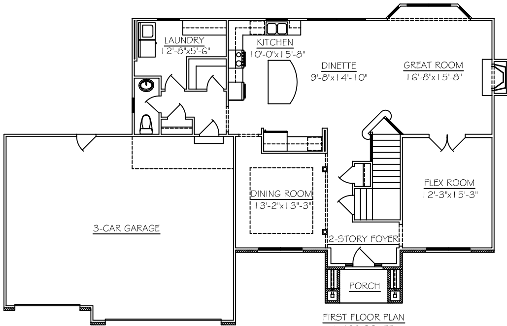
FIRST FLOOR PLAN 1,438 SQ. FT.
