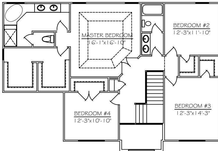
SECOND FLOOR PLAN 1,352 SQ. FT.
