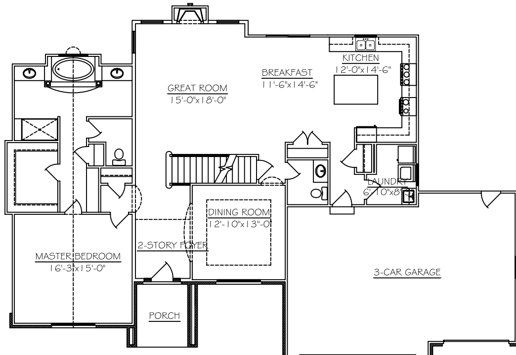
FIRST FLOOR PLAN 1,806 SQ. FT.
