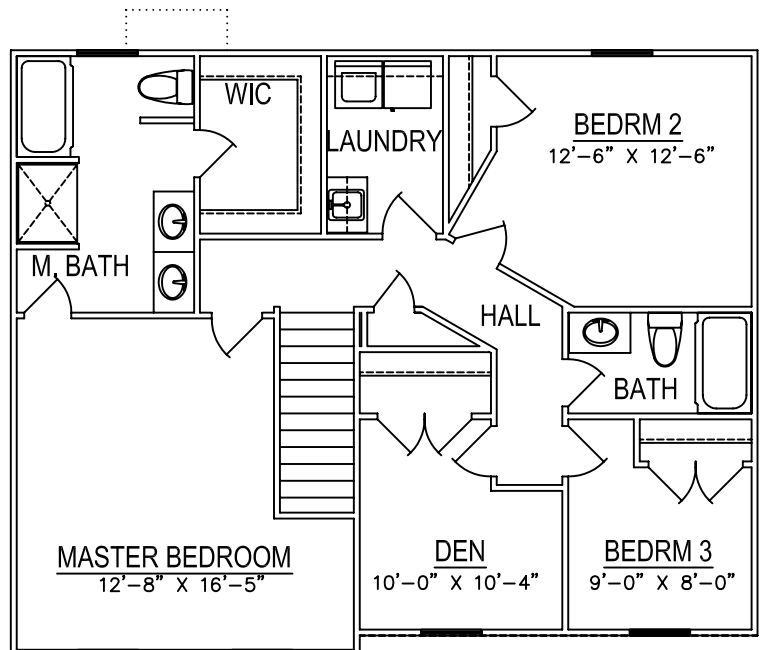
SECOND FLOOR PLAN 1,054 SQ. FT.
