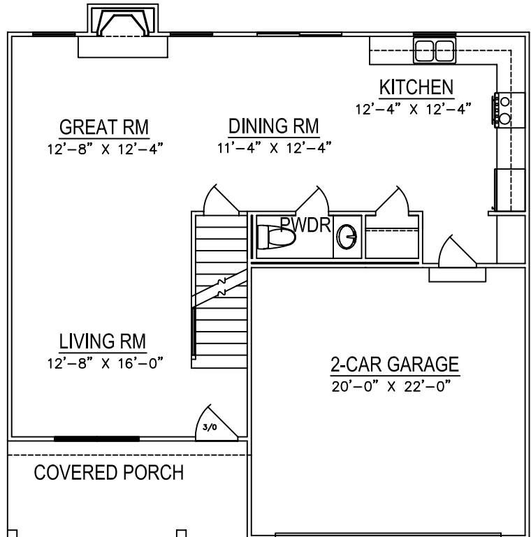
FIRST FLOOR PLAN 810 SQ. FT.
