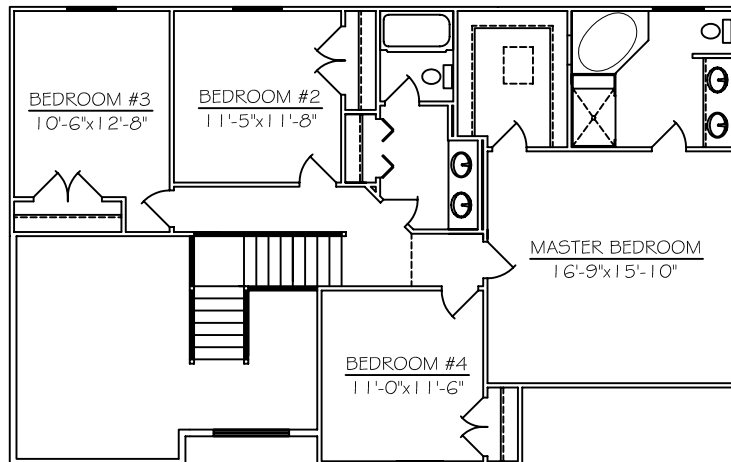
SECOND FLOOR PLAN 1,150 SQ. FT.
