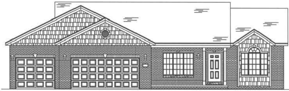
FRONT ELEVATION
