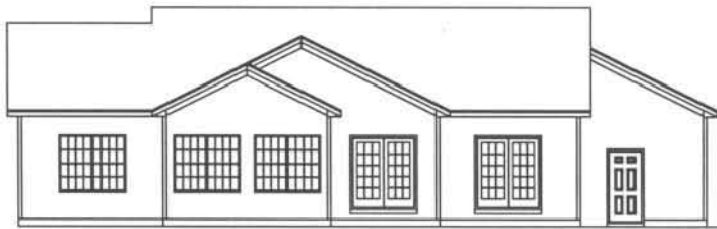
FRONT ELEVATION
