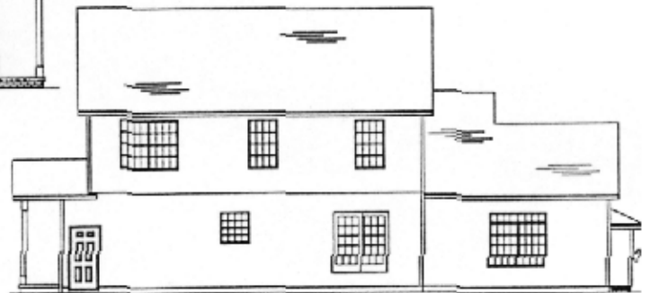
REAR ELEVATION
